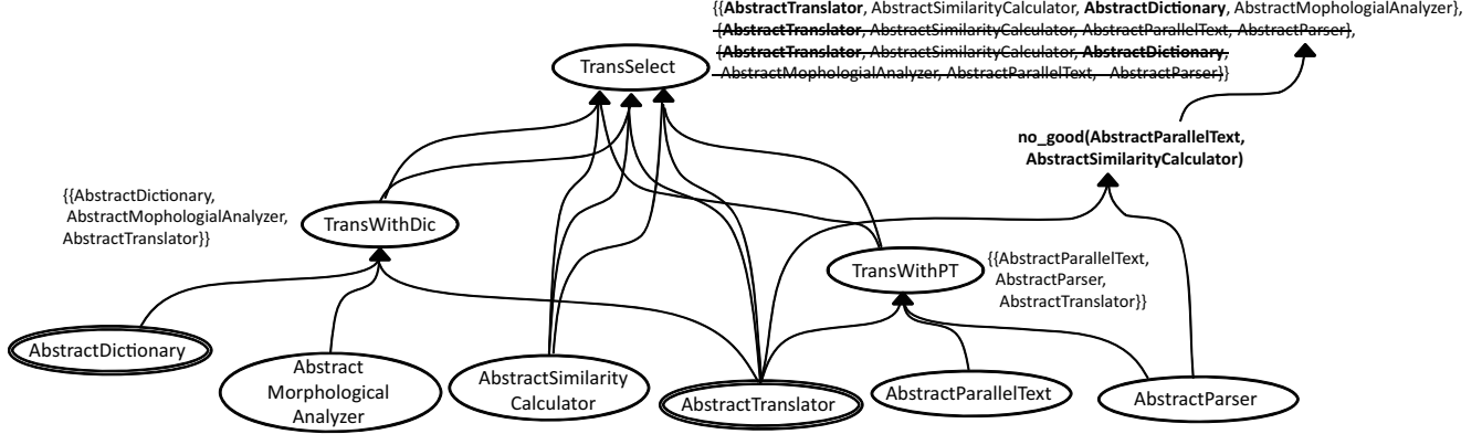
Figure 3. A binding dependency graph.
